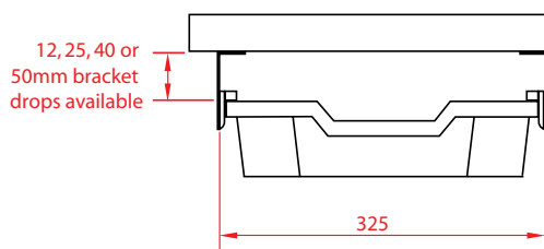
Single bracket
