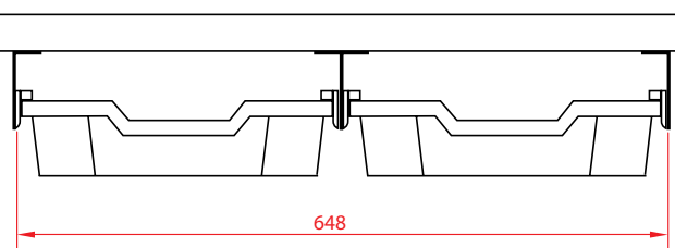
Double bracket
