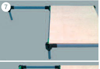
7 Repeat these steps until the entire stage is built.
