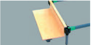
Steps and trims attach to the frame before the deck panel is located. It is advisable that they be situated before the panel is placed in any stage build to avoid trapping fingers.
