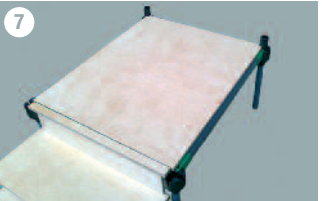
7 Once the second row is complete continue to build the base of the tiering block by using 450mm legs. Insert Tier Risers into each node along the base of the tiering block. Connect the riser cups of the third row (front and back) using 300mm legs, black and green rails.
