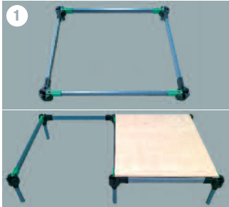
1 Using 150mm legs create the first row by assembling rails as per for a standard stage. Once the frame is complete add a single deck panel to 'Square' the unit. Then continue to build until the first row is completed.
