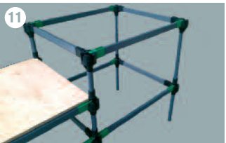
11 Any further rows from this will be based upon this structural format. For example: a fifth row would be 450mm legs, 600mm legs and 300mm legs down the rear whilst a sixth would be 450mm, 600mm and 600mm legs.
