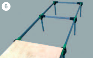
6 Once any necessary steps and trims are in place fit the deck to the second row unit and continue building the second row in this way until complete.
