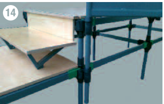
14 Insert the leg of the handrail through both adapters. Note; It is easier to hold the deck bar at 45° to the tiering in order to swing the clasps onto the adapters on the next level.
